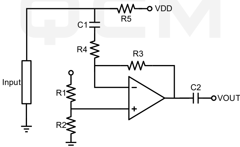
Figure 1. Typical Application
